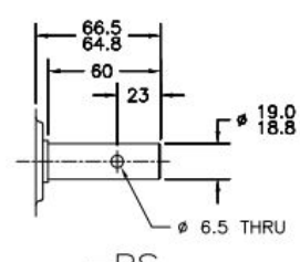
SEE DWG. M164-1RS USE #8648 OIL SEAL
