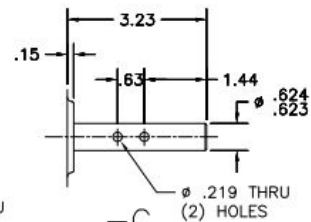
SEE DWG. M164-1C USE #6372 OIL SEAL
