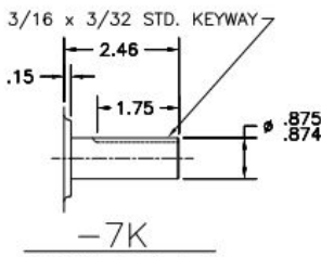
SEE DWG. M164-1-7K USE #8648 OIL SEAL
