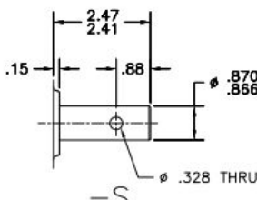
SEE DWG. M164-1S USE #8648 OIL SEAL
