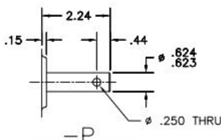
SEE DWG. M164-1P USE #6372 OIL SEAL
