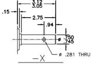
SEE DWG. M164-1X USE #8648 OIL SEAL
