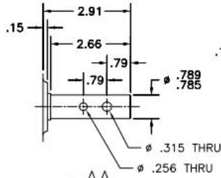
USE #8648 OIL SEAL SEE DWG. M164-1AA
