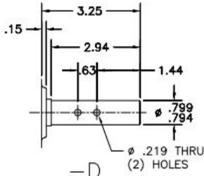
SEE DWG. M164-1D USE #8648 OIL SEAL
