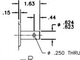
SEE DWG. M164-1R USE #6372 OIL SEAL
