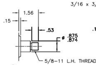
SEE DWG. M164-1J USE #8648 OIL SEAL
